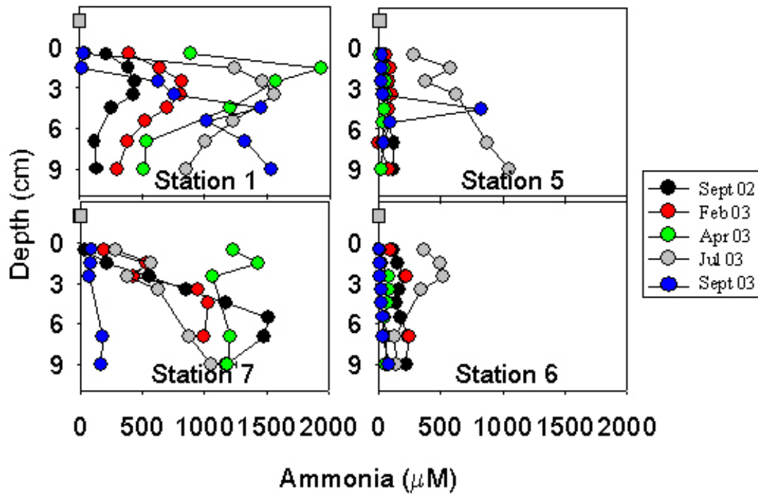
Figure 15: Vertical profile of pore water \text{NH}_4 concentration by site and season.
