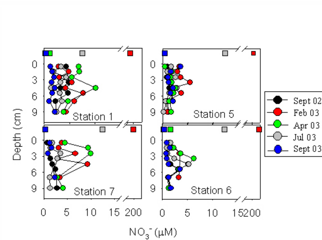
Figure 17: Vertical profile of pore water \text{NO}_3^- concentration by site and season
