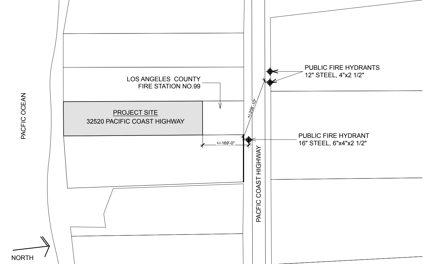
FIRE HYDRANT LOCATION PLAN
