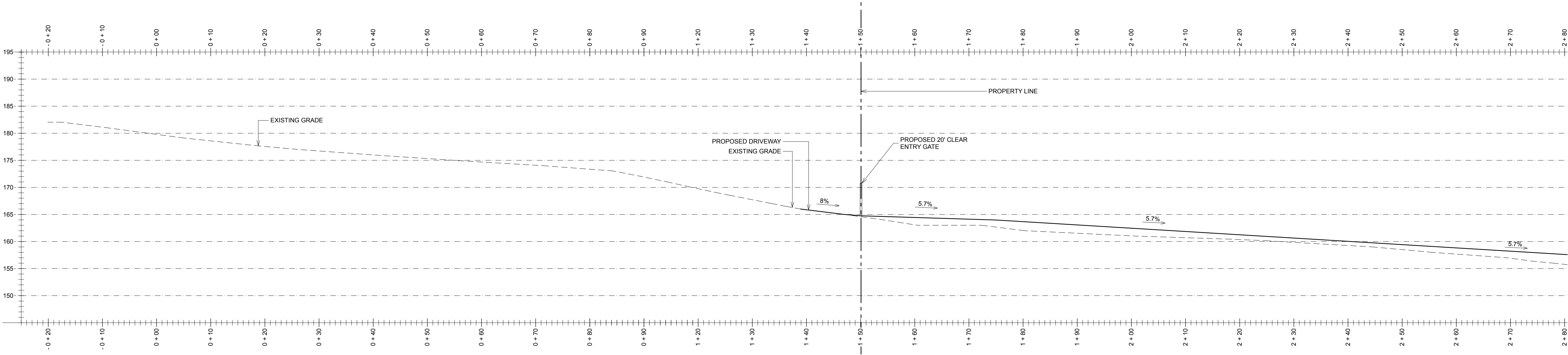
FIRE DEPT - MAIN HOUSE DRIVEWAY PROFILE A
