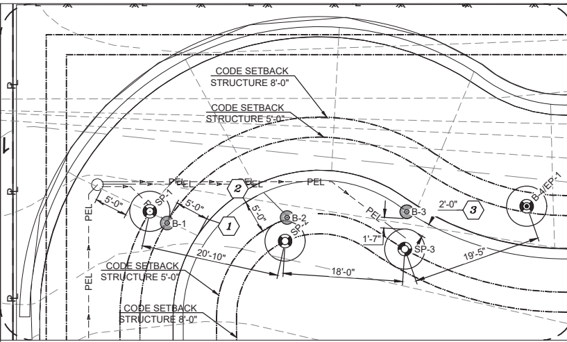
2 DETAILED SETBACK AND SEEPAGE PIT PLAN 1"=20'
