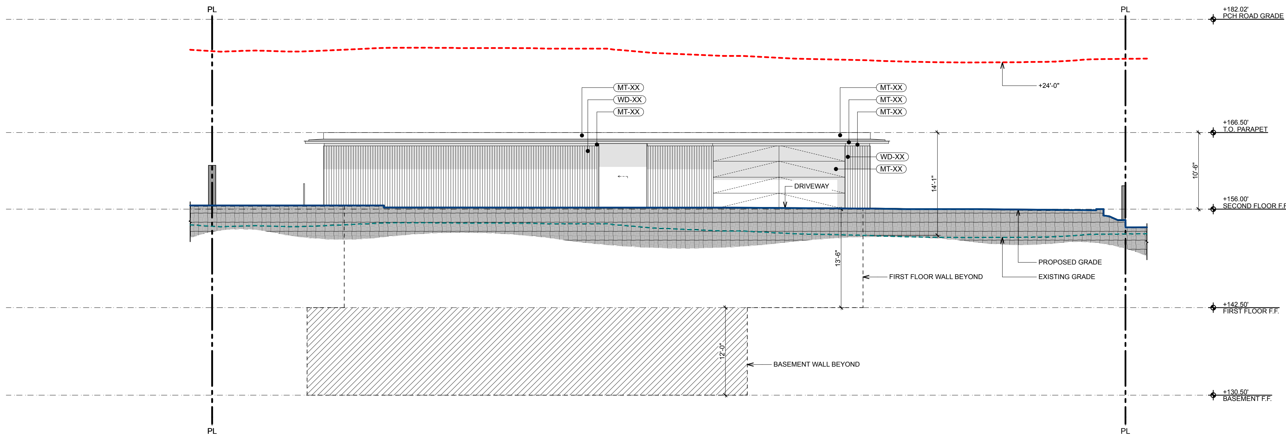
MAIN HOUSE - NORTH ELEVATION 01
