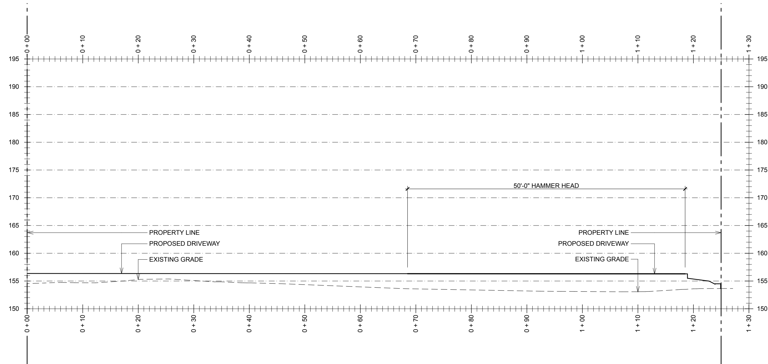
FIRE DEPT - MAIN HOUSE DRIVEWAY PROFILE B
