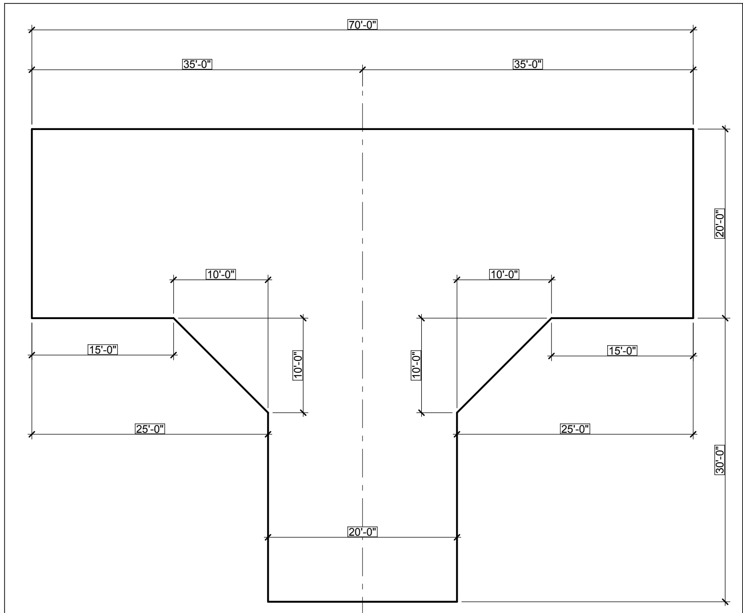
APPARATUS HAMMERHEAD TURNAROUND
