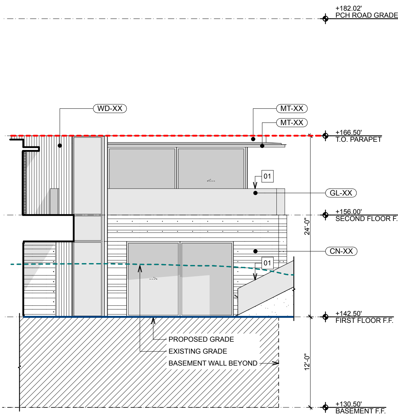
MAIN HOUSE - COURTYARD - SOUTH ELEVATION 05
