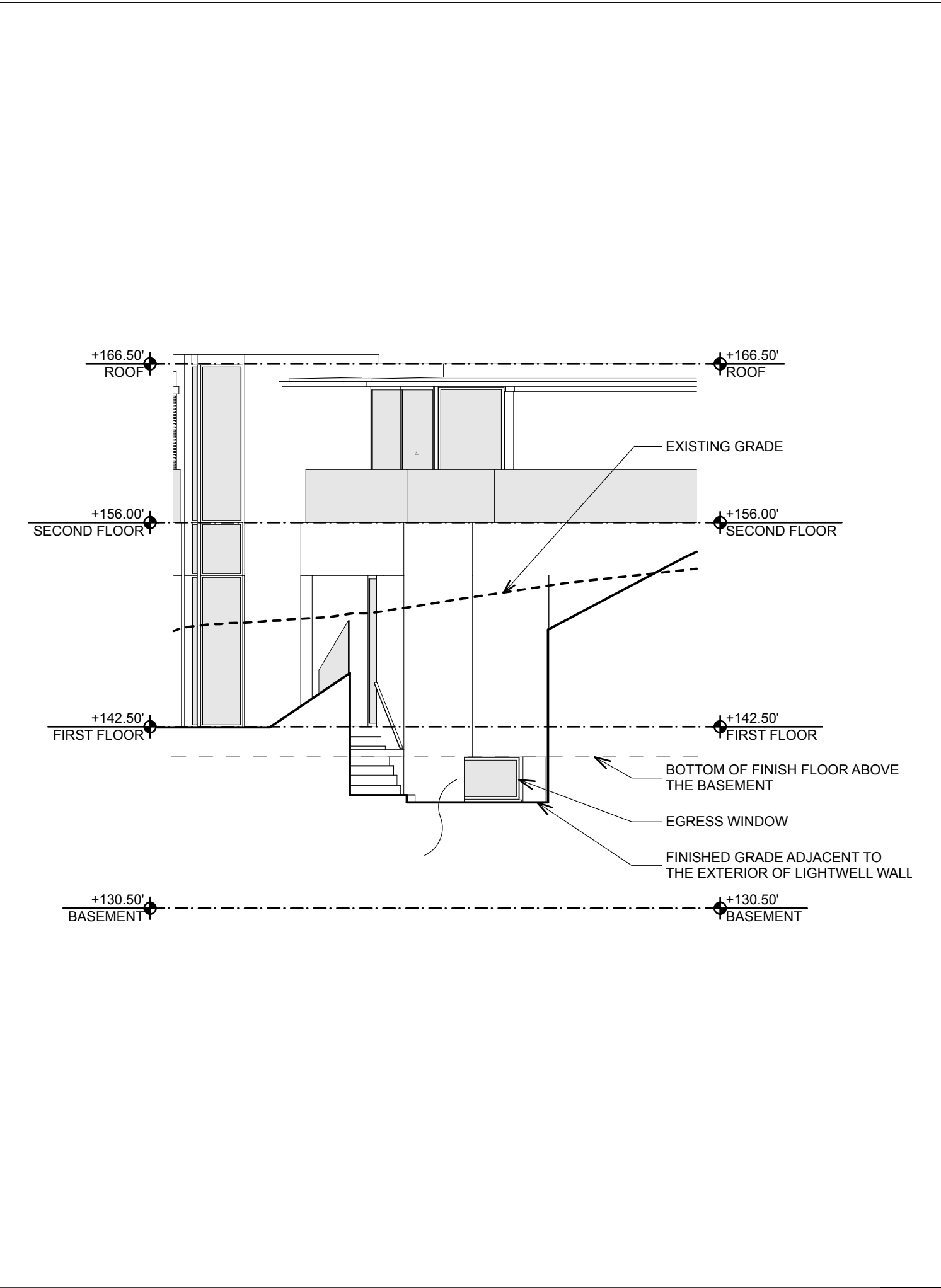
MAIN HOUSE - EGRESS WELL SECTION 04
