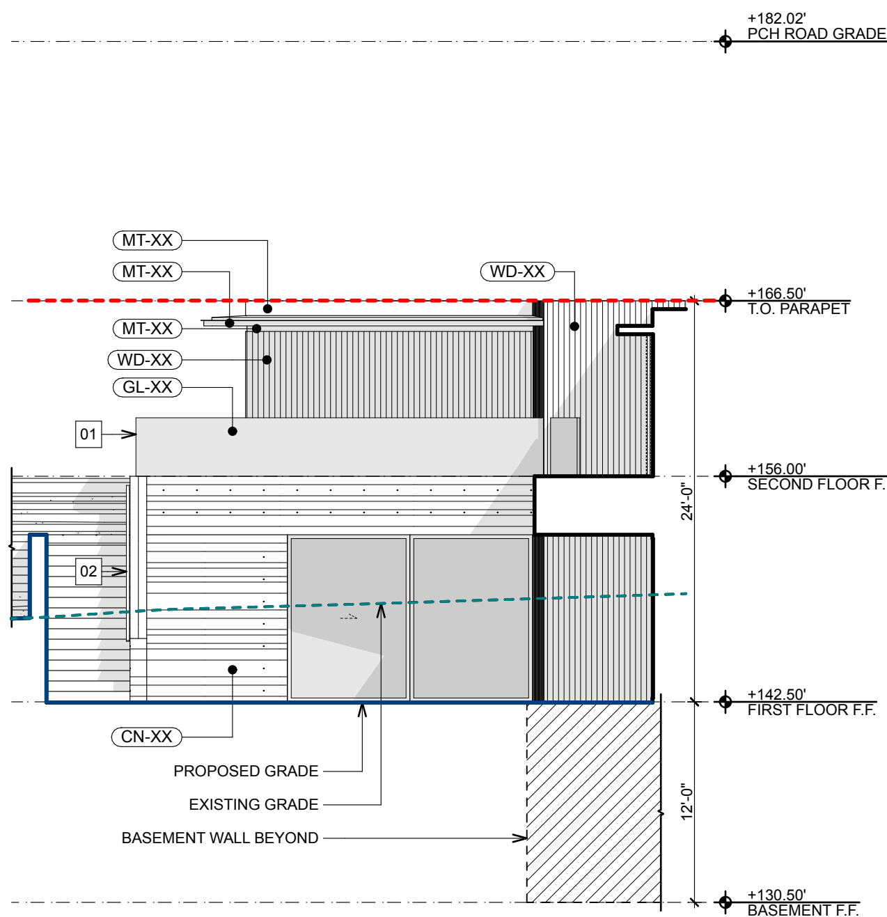
MAIN HOUSE - ENTRY COURTYARD - SOUTH ELEVATION 06
