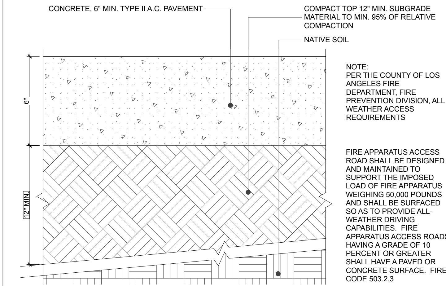
VEHICULAR PAVING DETAIL
