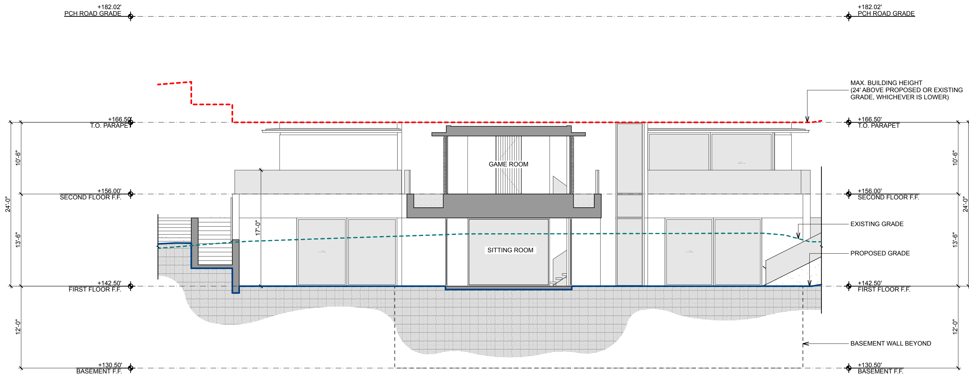
MAIN HOUSE - BUILDING SECTION 01
